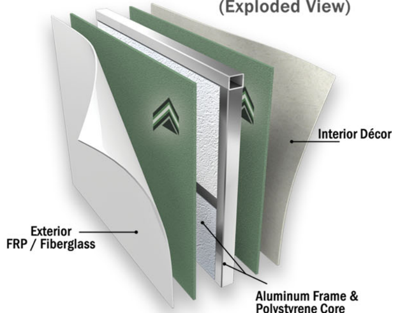
RV Sidewall Cut-Away (Exploded View)
